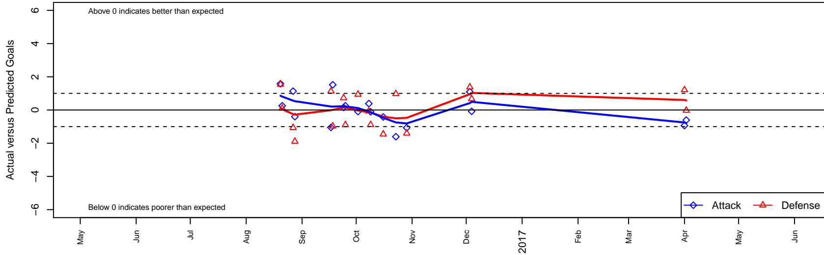
LA Galaxy South Bay Elite B02 Dots are actual minus expected GF (blue circles) and GA (red triangles). Blue line is smoothed change in attack strength. Red is smoothed change in defense strength.
